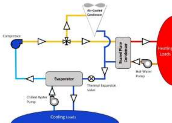
Figure 4 - Heat Recovery
