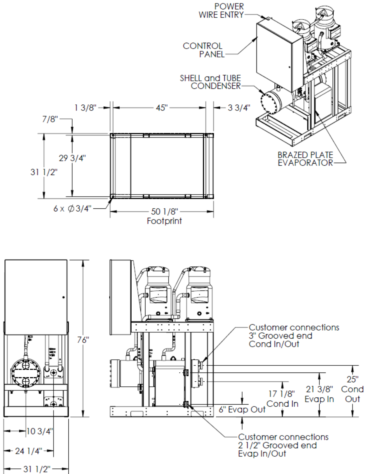
Figure 16 - No Header Piping, Shell & Tube Condenser (Standalone Chiller Application)
