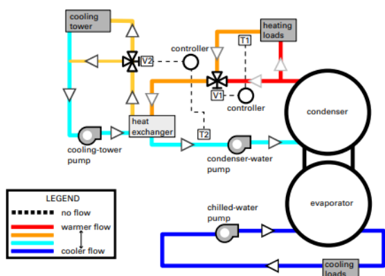
Figure 4 - Heat Recovery
