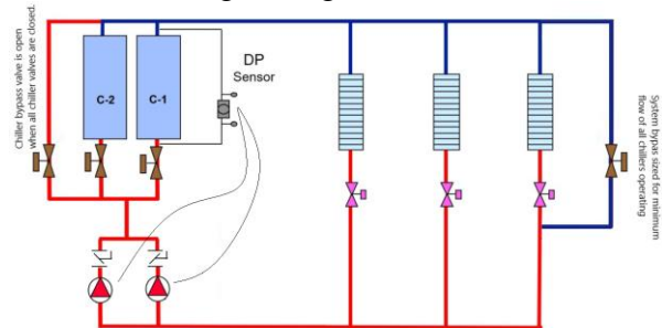
Figure 6- Variable Flow with Parallel Pumps
