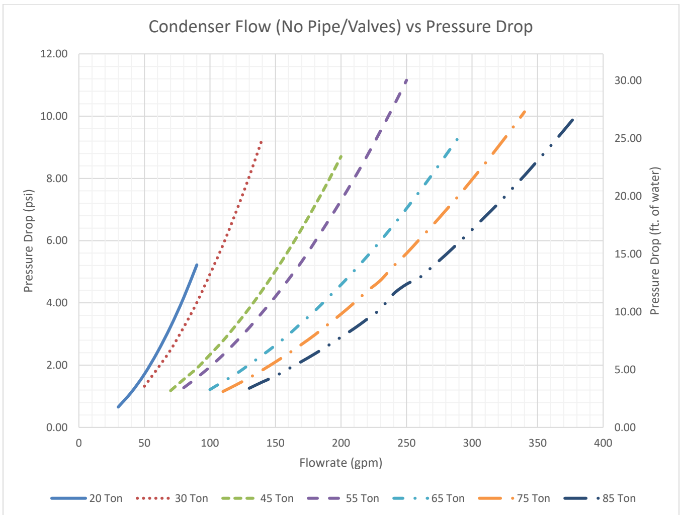
Figure 11- Brazed Plate Condenser Flow (heat exchanger only) vs. Pressure Drop
