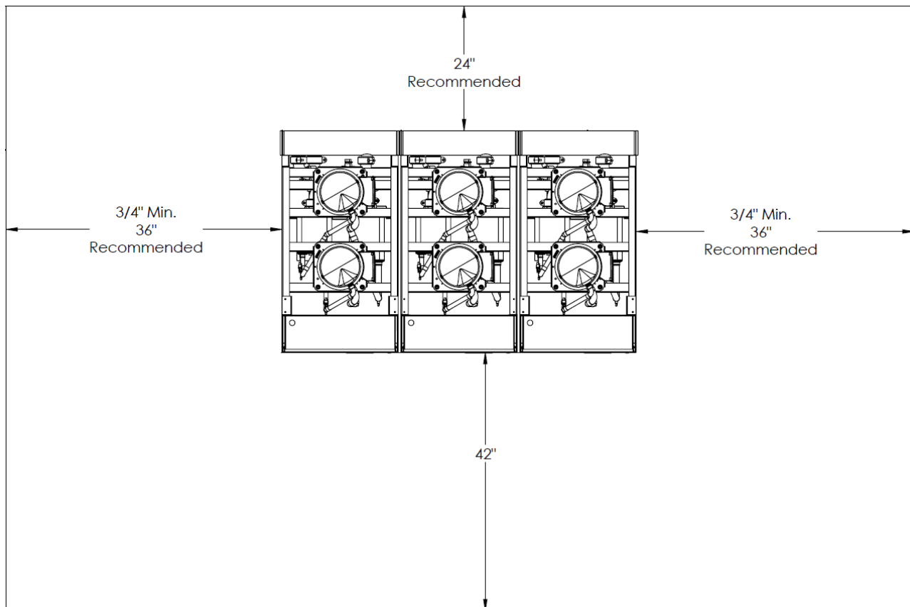
Figure 14 – Recommended Service Clearances
