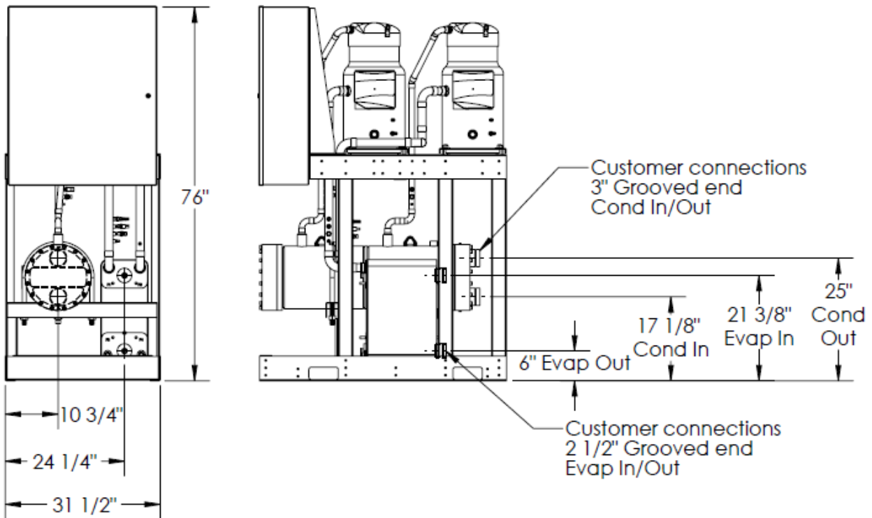
Figure 16 - No Header Piping, Shell & Tube Condenser (Standalone Chiller Application)
