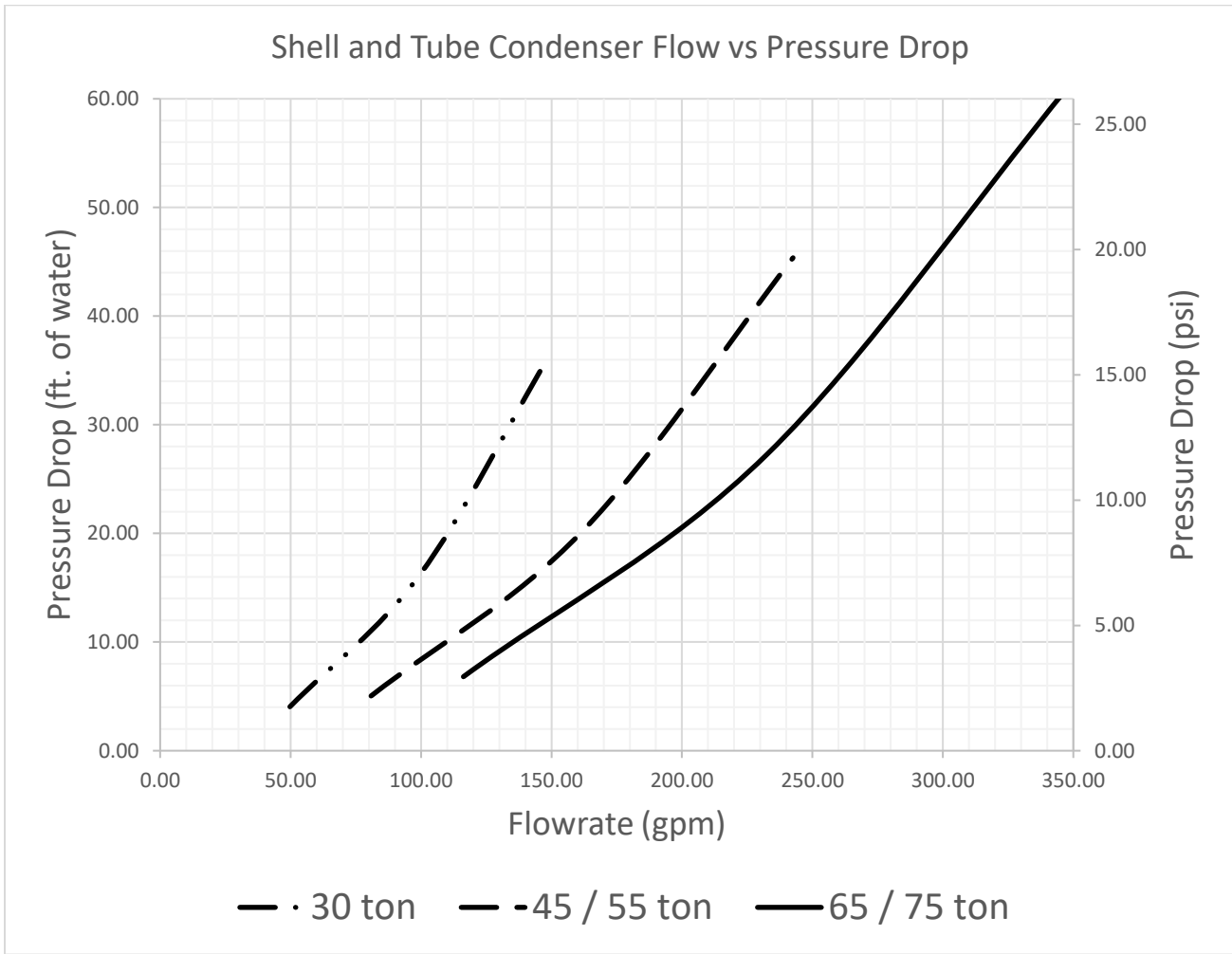
Figure 12- Shell and Tube Flow (including header and valves) vs. Approximate Pressure Drop
