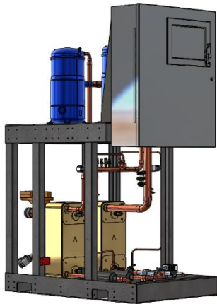
Figure 9 - No Header, Heat Exchangers Only Configuration
