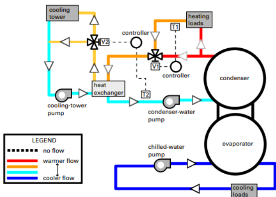
Figure 4 - Heat Recovery
