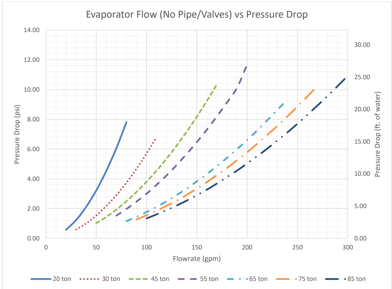
Figure 10- Evaporator Flow (heat exchanger only) vs. Pressure Drop
