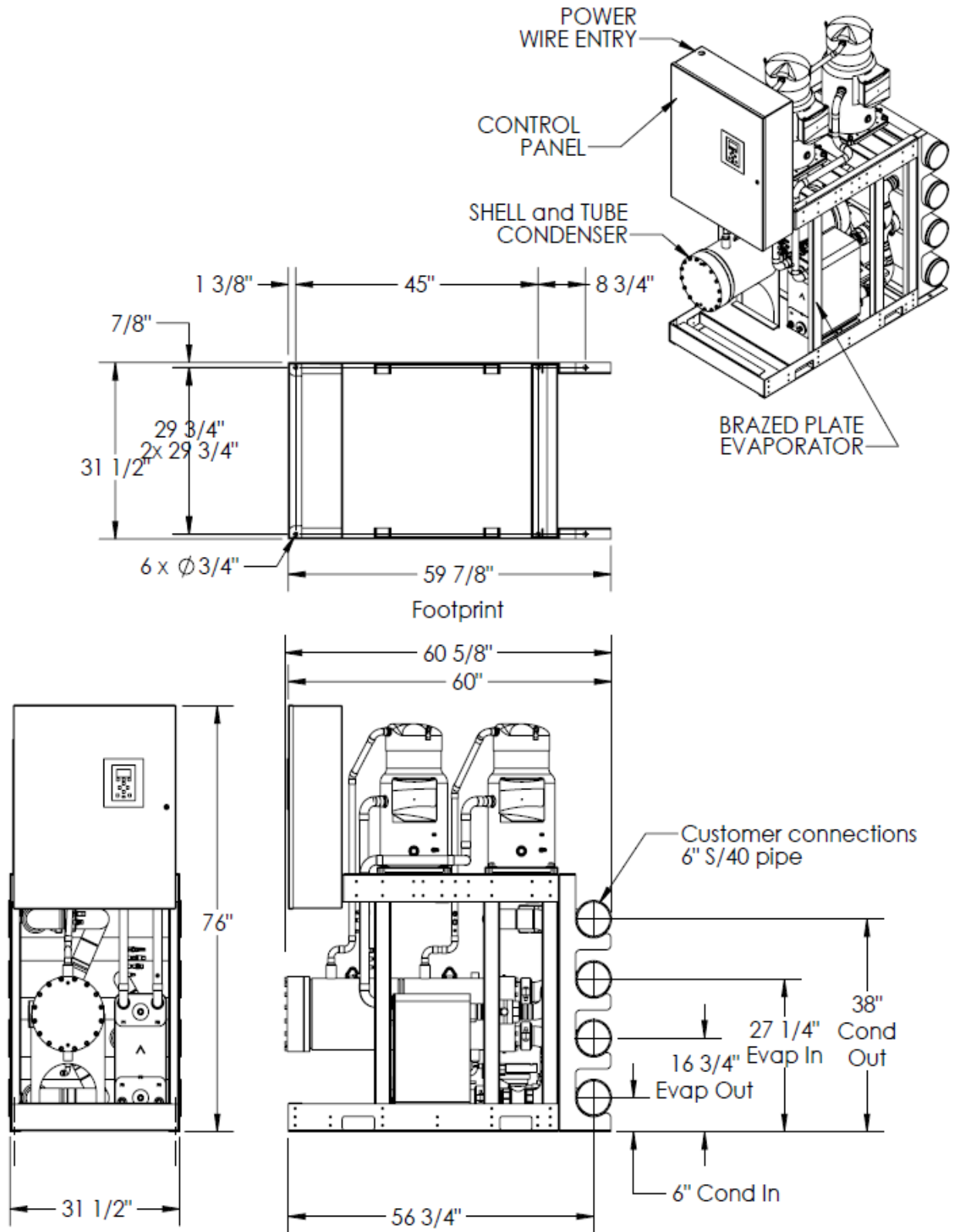
Figure 18 - Shell and Tube Condenser (Array application)
