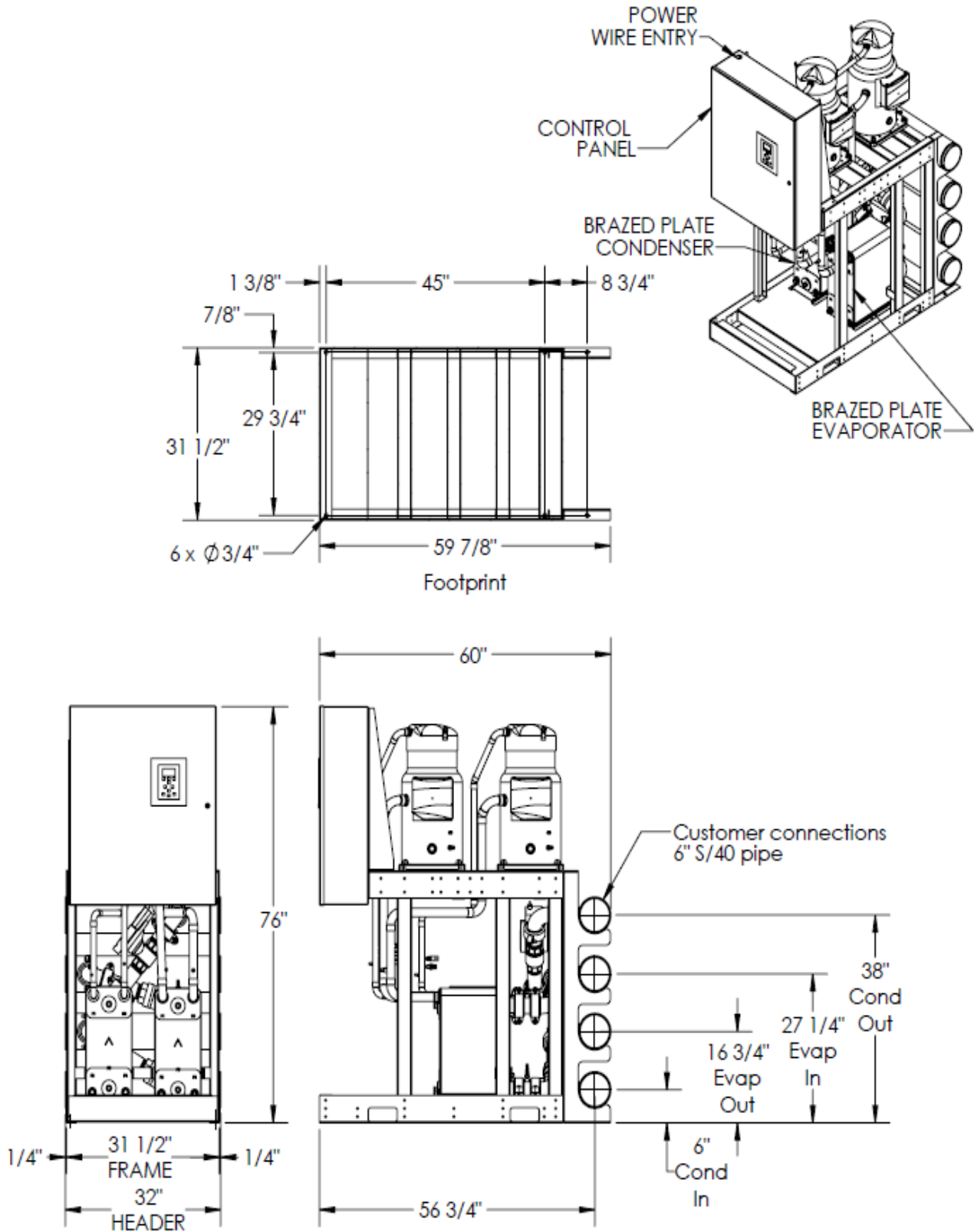
Figure 17 - Header Piping, Brazed Plate Condenser (Array application)
