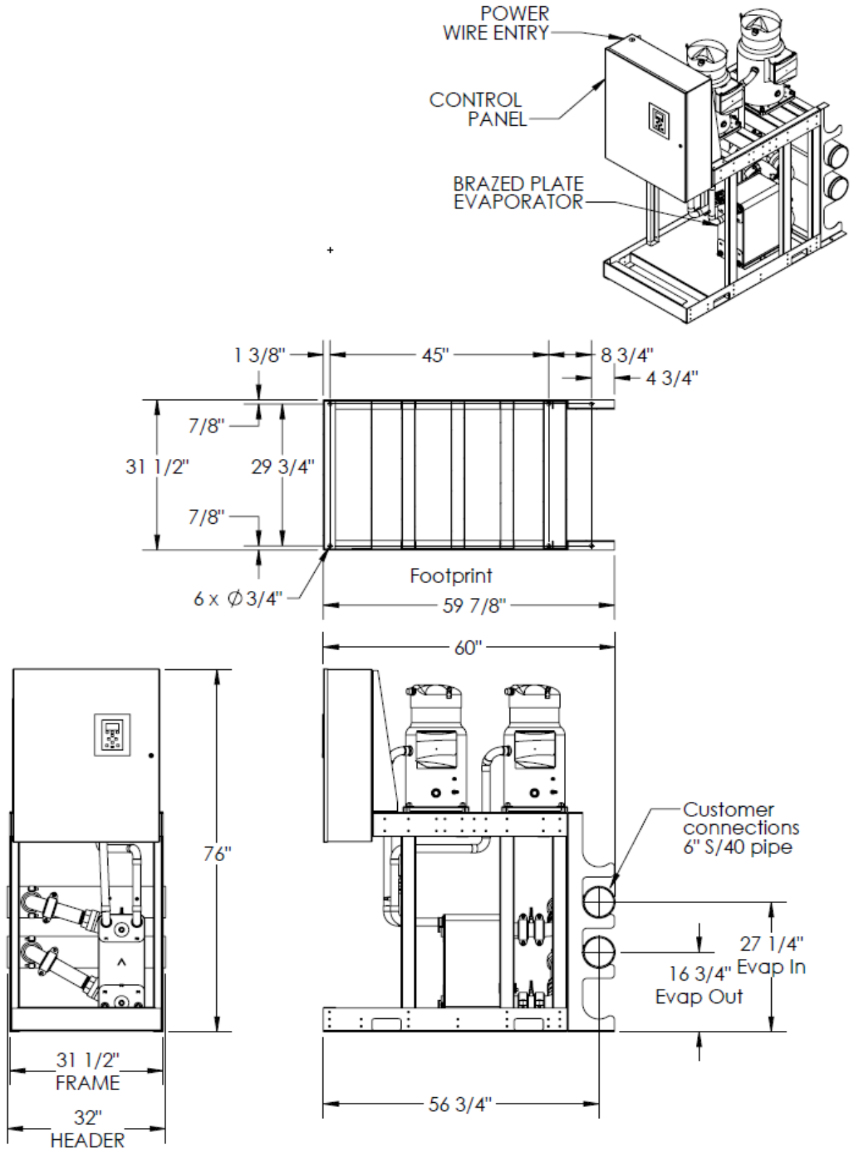
Figure 19 - Remote Air-Cooled Condenser (Array application)
