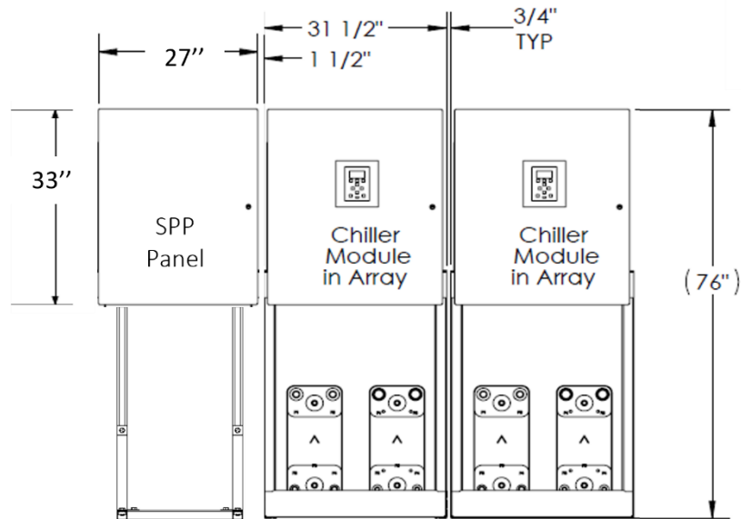
Figure 12- Single Point Power Distribution Panel Estimated Dimensions
