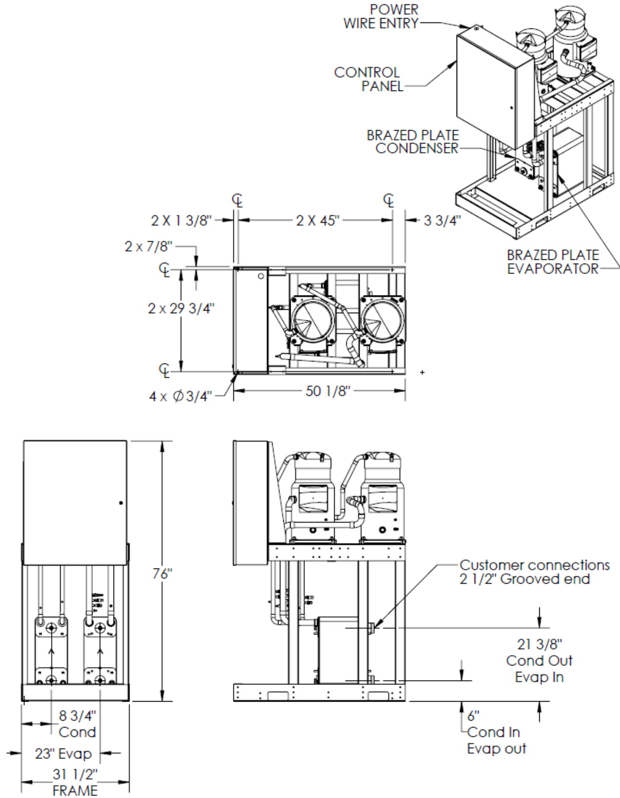
Figure 15 - No Header Piping, Brazed Plate Condenser (Standalone Chiller Application)
