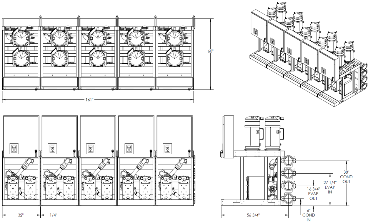
Figure 20 - Example Array Dimensions
