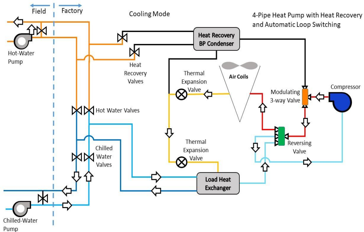
Figure 8. Four-Pipe Cooling Mode Operation
