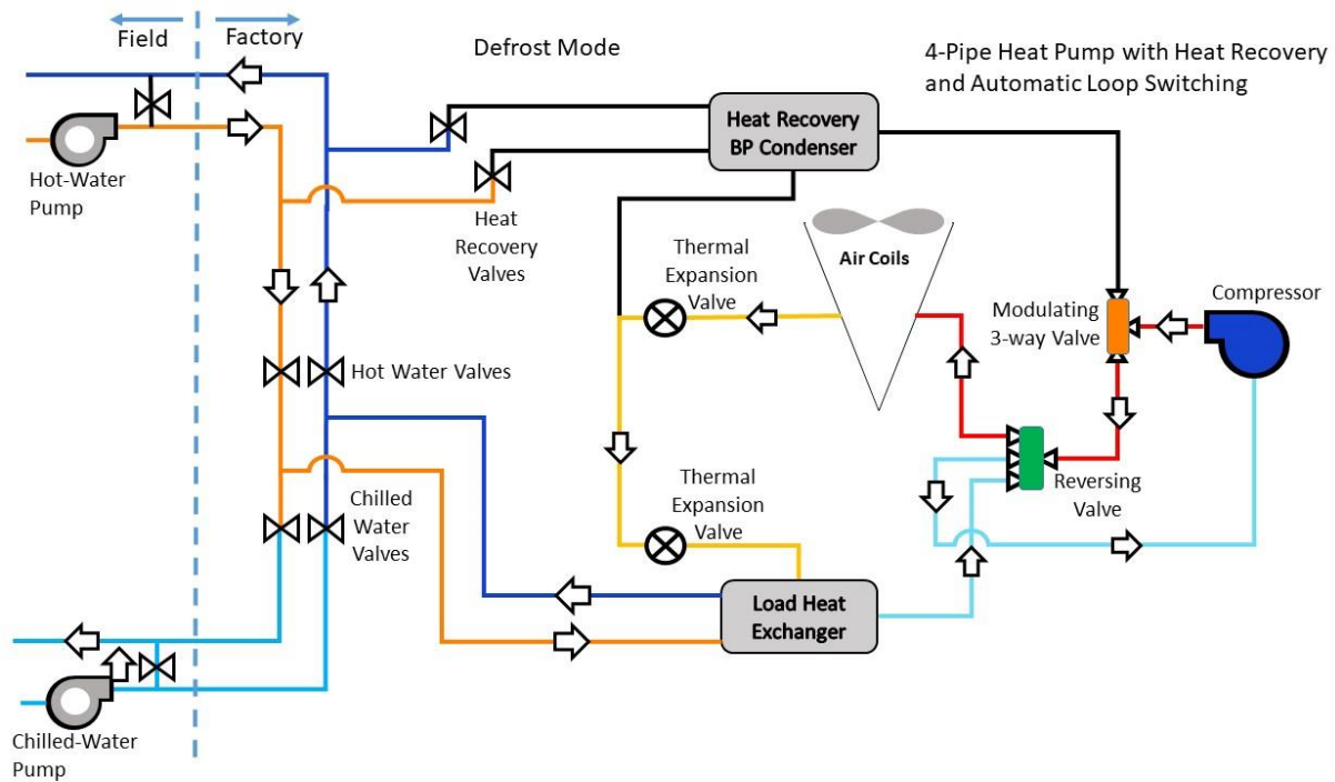
Figure 9. Four-Pipe Defrost Operation Mode
