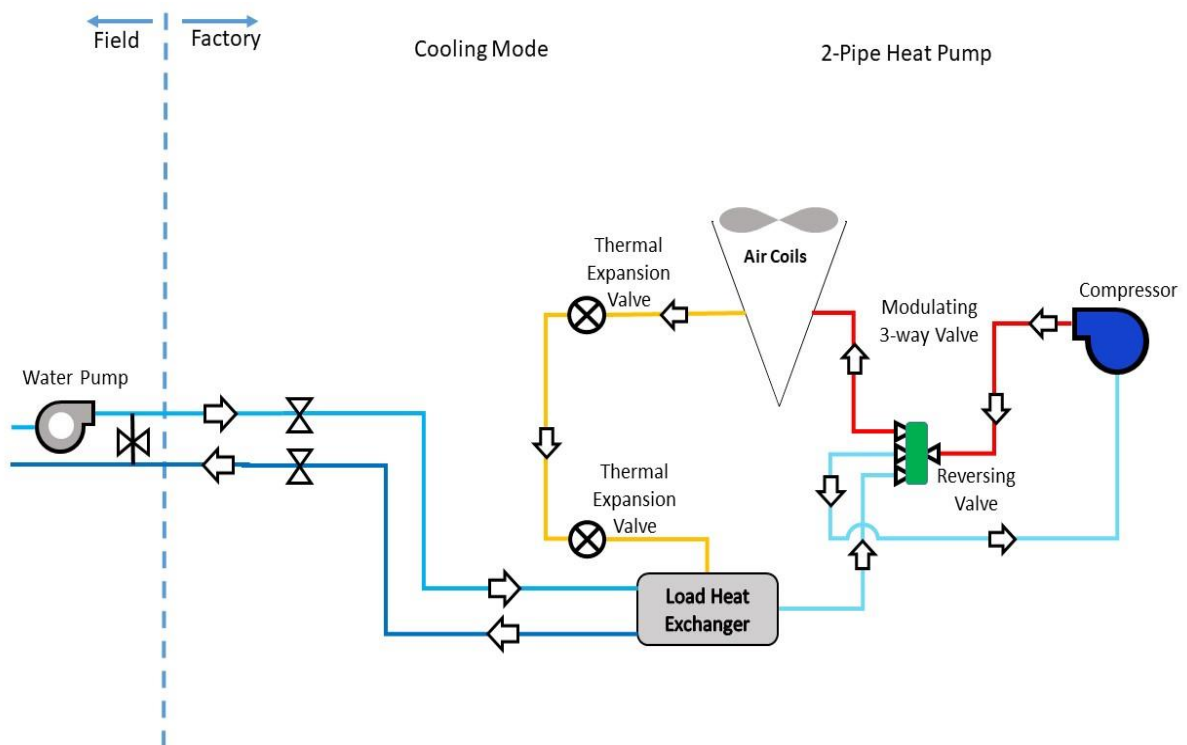
Figure 2. Cooling Mode Operation
