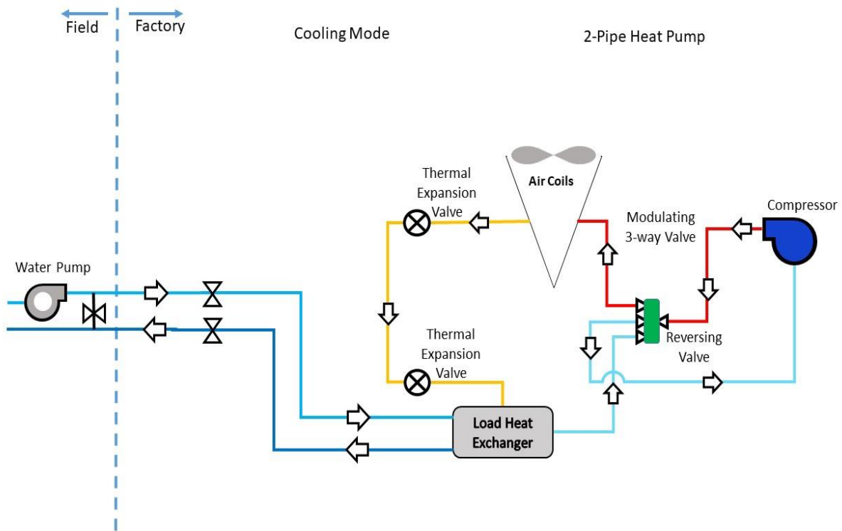
Figure 4. Defrost Cycle Operation
