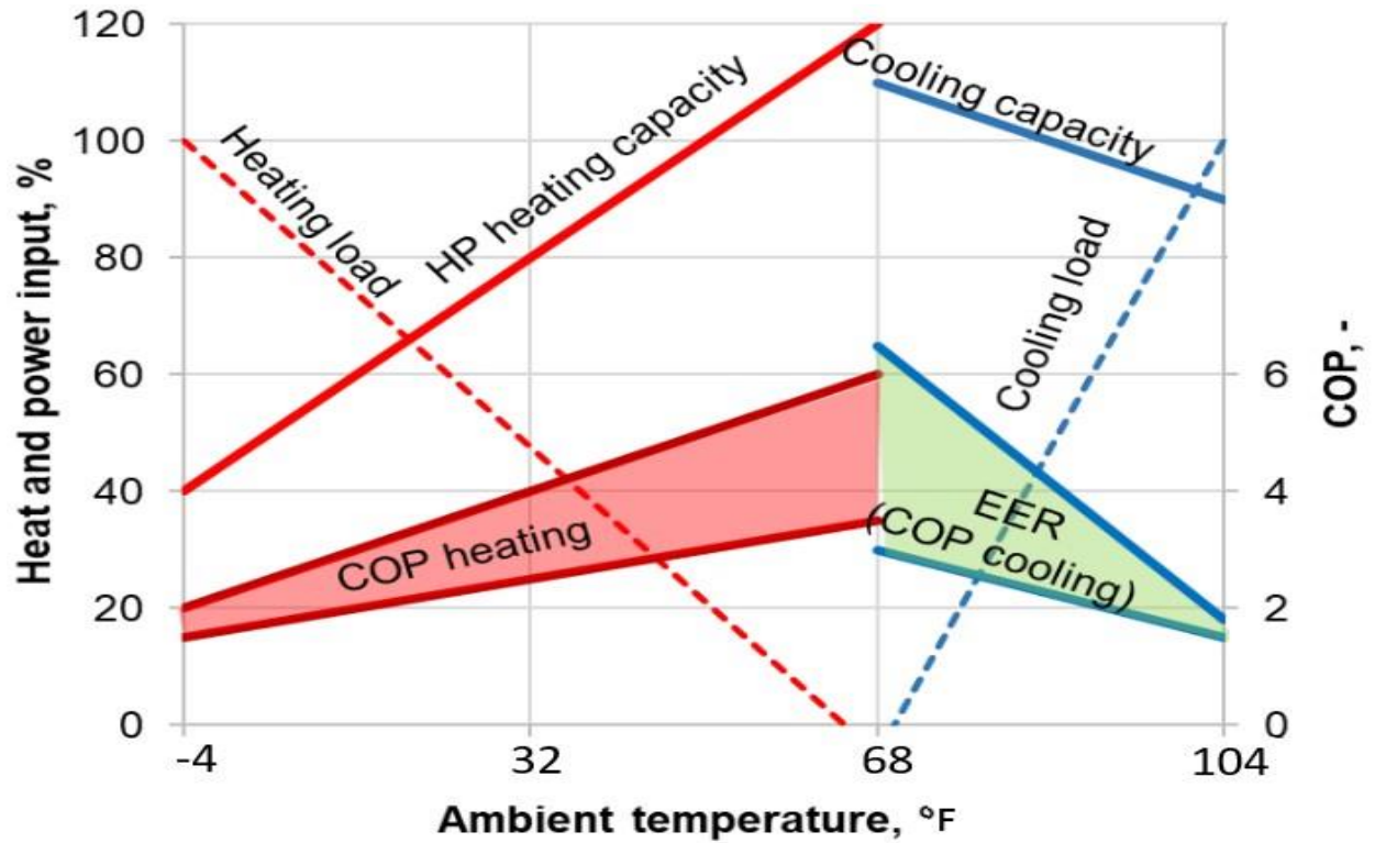
Figure 10. Ambient impact on heat pump leaving water temperature
