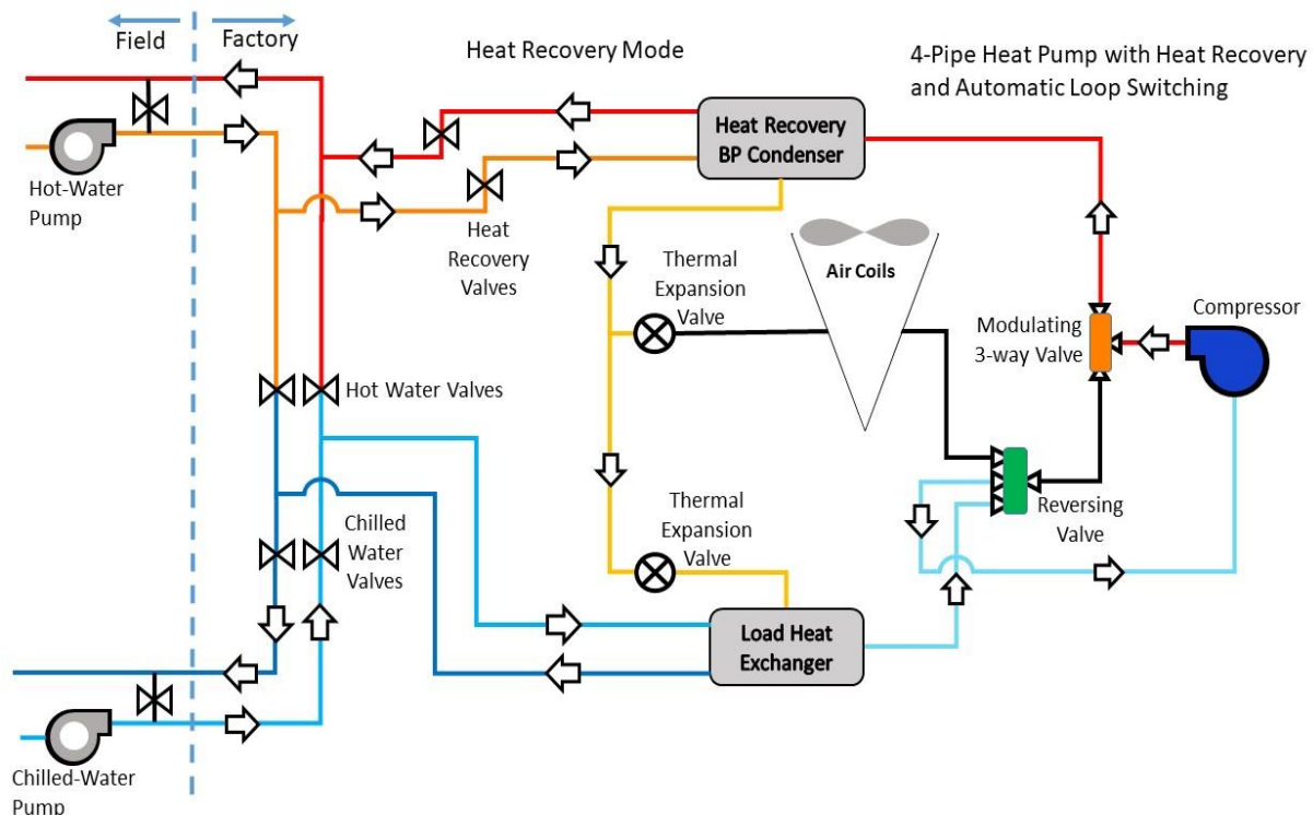
Figure 6. Four-Pipe Heat Recovery Mode Operation
